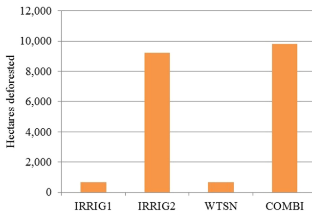
Fig. 5. Scenario impacts on cumulative deforestation in hectares between 2030 and 2017. Source: IEEM Platform results.
