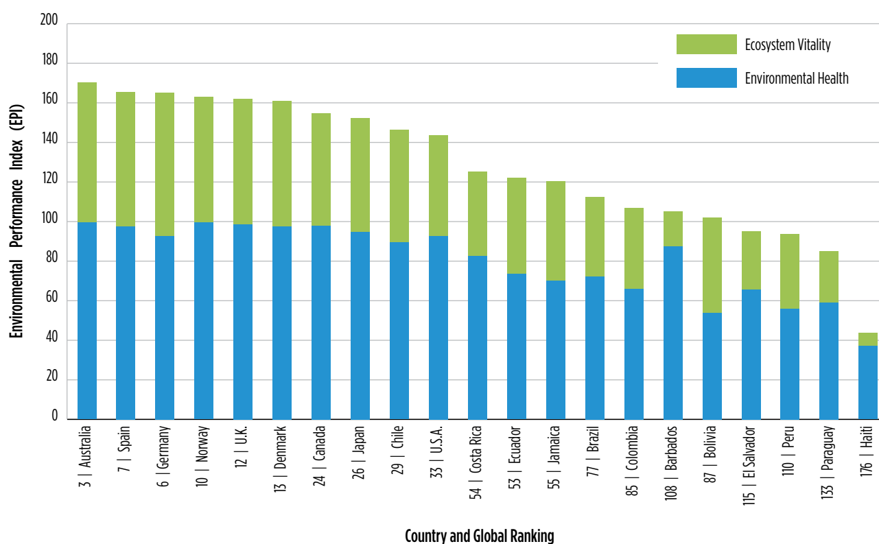
Figure 1. Environmental Performance Index for 2014
