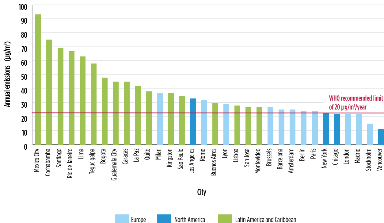
Figure 4. Annual PM 10 (µg/m 3 ) emissions in LAC, European, and North American cities
